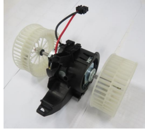
BLOWER ASSY
